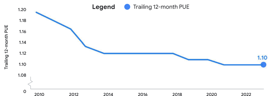
FIGURE 3 Energy efficiency at Google data centers
